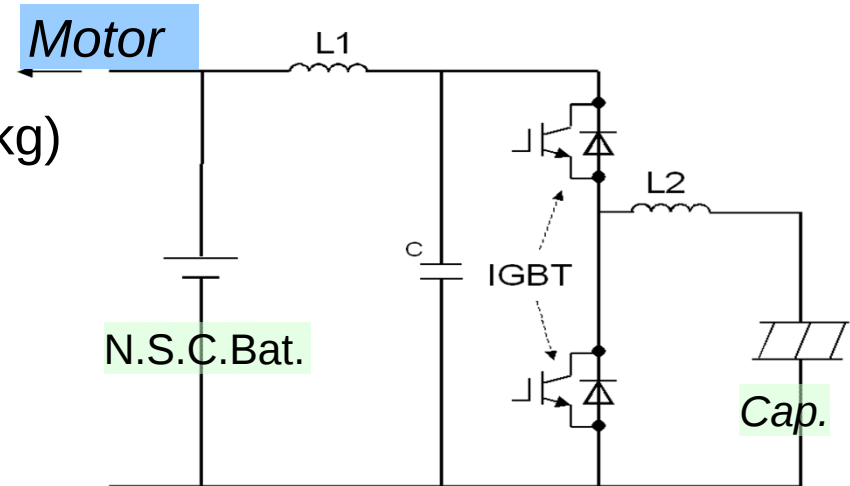
Battery & S. Capacitor Hybrid Power System
